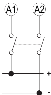
Fig. 1 Power supply
